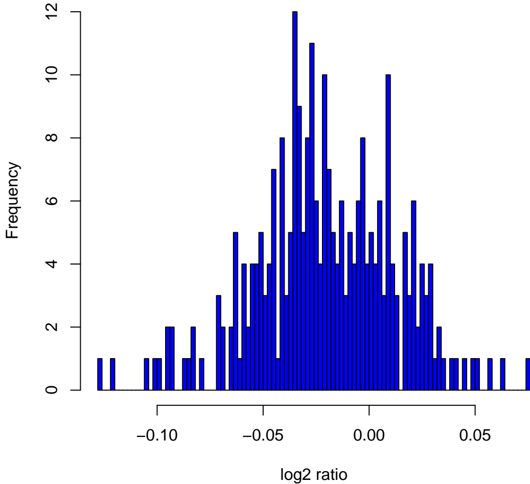
Histogram of log 2 ratios in 270 HapMap samples at clone Chr6tp-15H6
