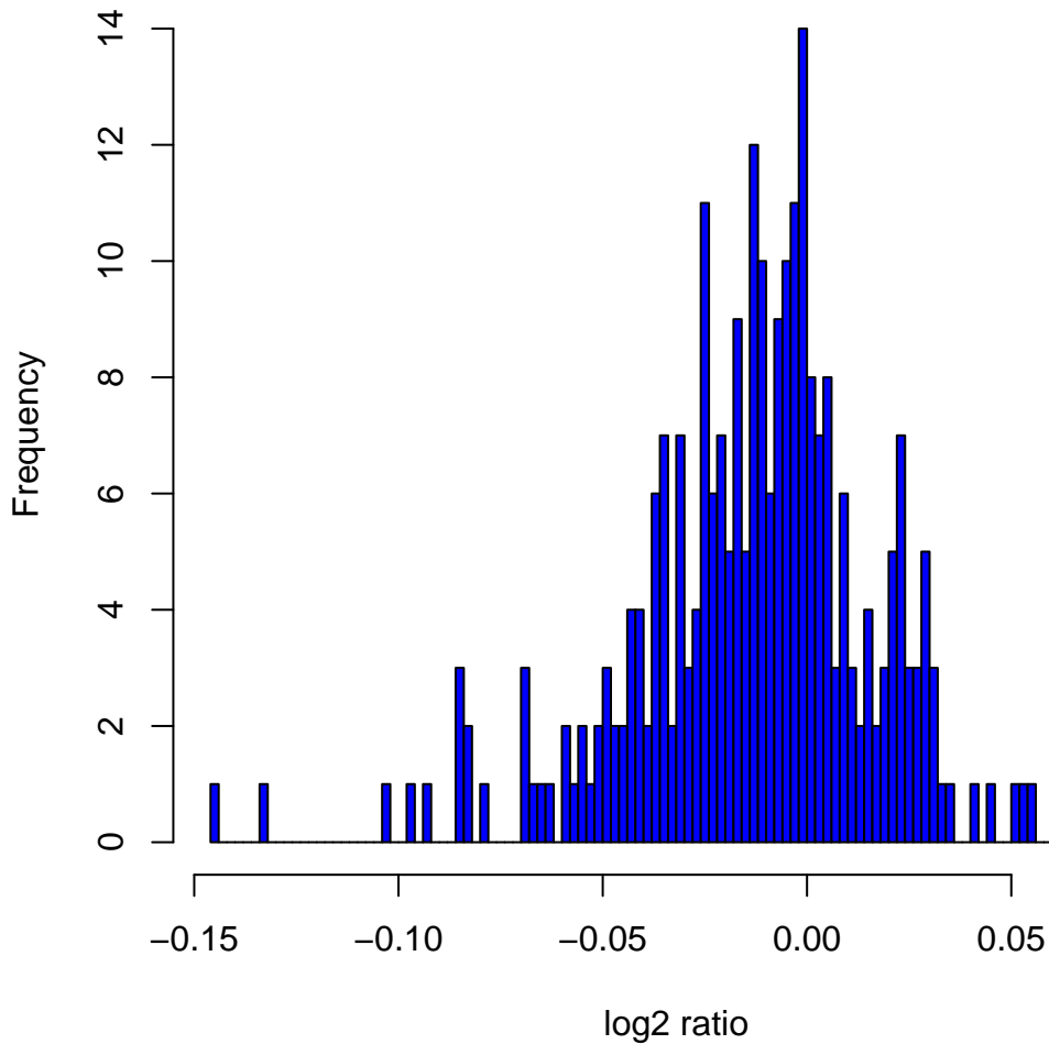
Histogram of log2ratios in 270 HapMap samples at clone Chr6tp-16A12
