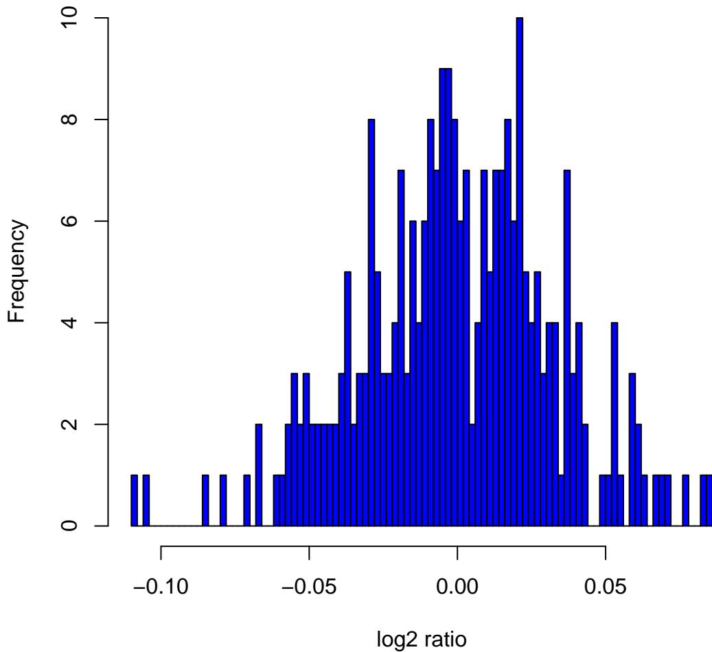
Histogram of log2ratios in 270 HapMap samples at clone Chr6tp-16H2
