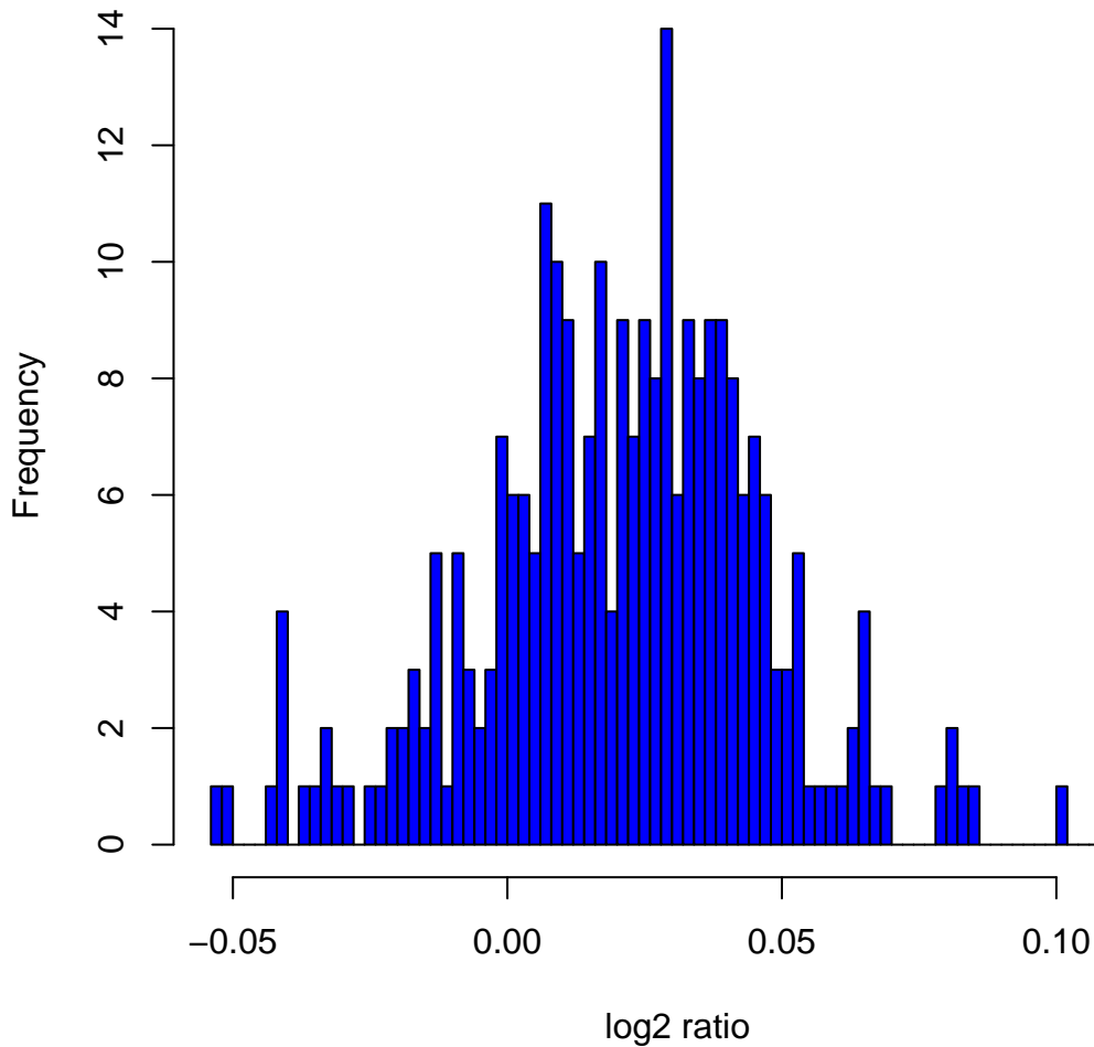
Histogram of \log_2 ratios in 270 HapMap samples at clone Chr6tp-17A7
