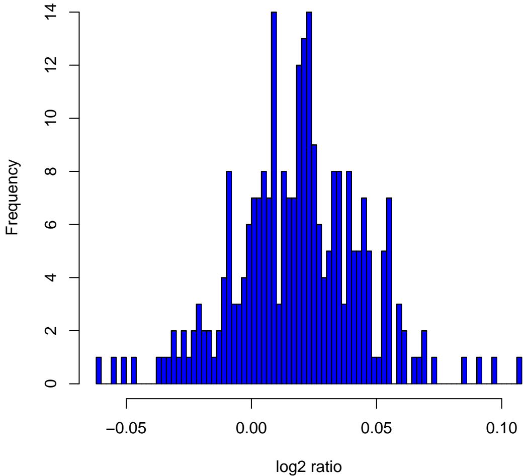
Histogram of log2ratios in 270 HapMap samples at clone Chr6tp-17D11
