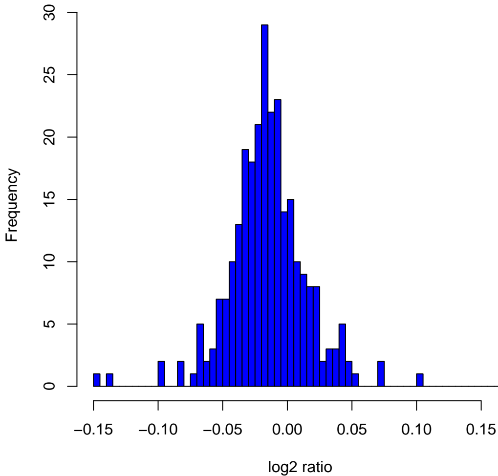
Histogram of \log_2 ratios in 270 HapMap samples at clone Chr6tp-17E7
