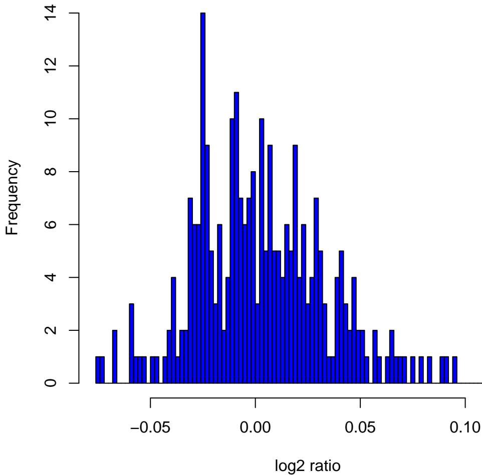
Histogram of \log_2 ratios in 270 HapMap samples at clone Chr6tp-17G11
