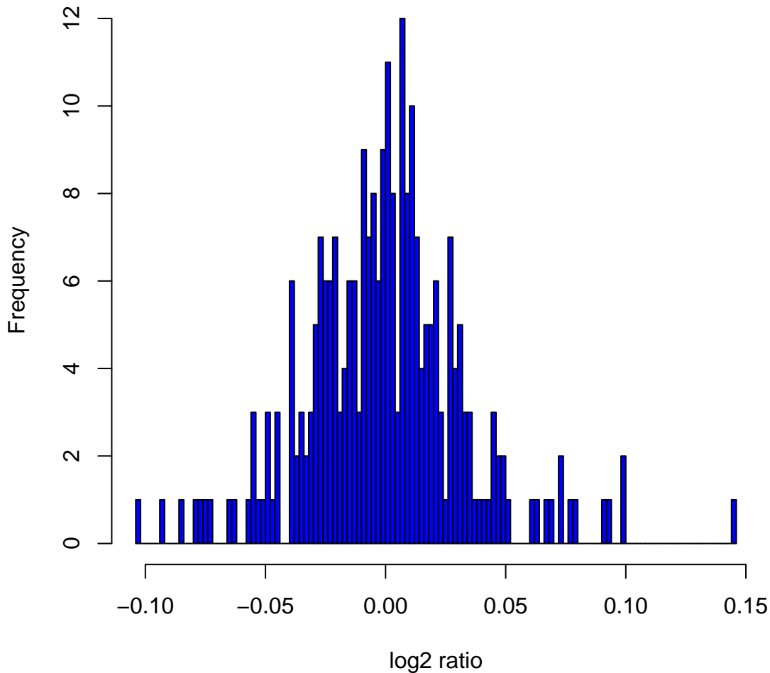
Histogram of log 2 ratios in 270 HapMap samples at clone Chr6tp-18A5
