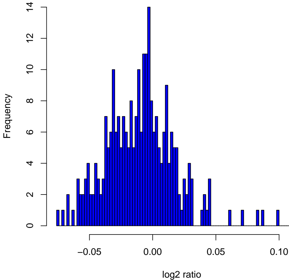
Histogram of \log_2 ratios in 270 HapMap samples at clone Chr6tp-18A8
