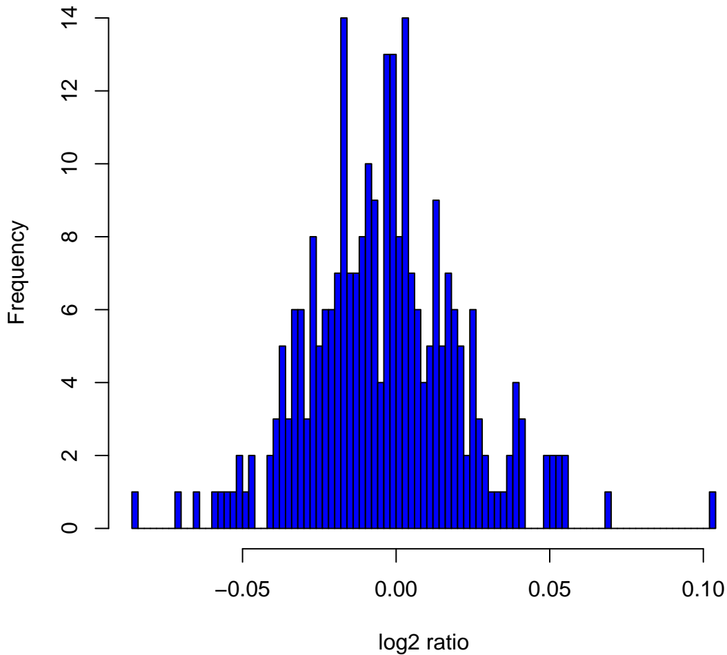
Histogram of log 2 ratios in 270 HapMap samples at clone Chr6tp-18E2
