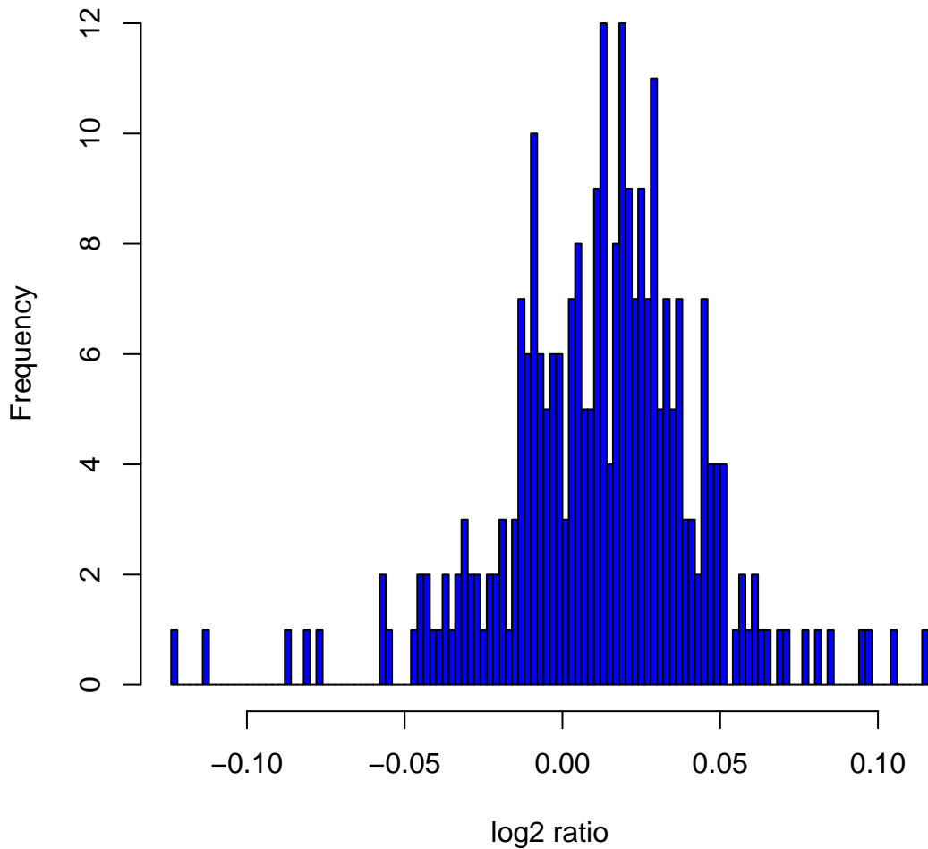
Histogram of log2ratios in 270 HapMap samples at clone Chr6tp-19C12
