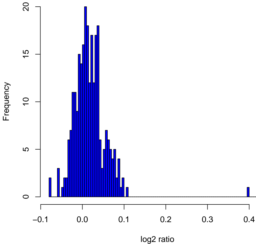
Histogram of log2ratios in 270 HapMap samples at clone Chr6tp-19E12
