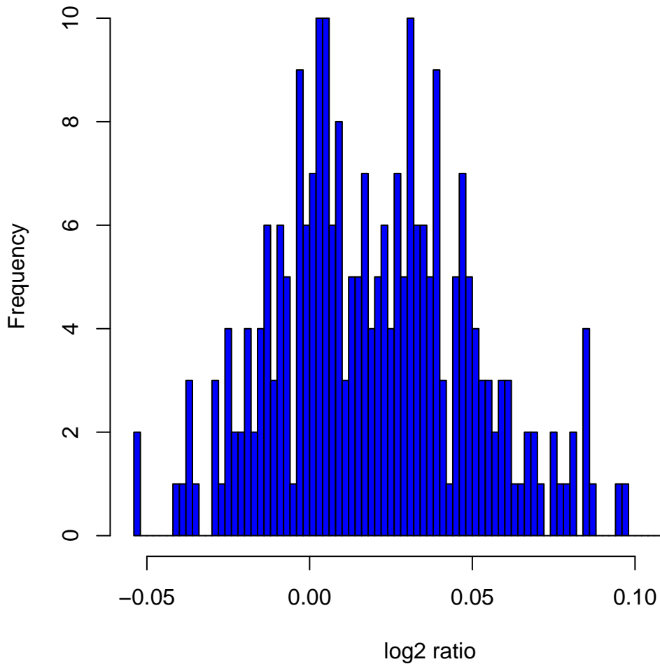
Histogram of \log_2 ratios in 270 HapMap samples at clone Chr6tp-19F1
