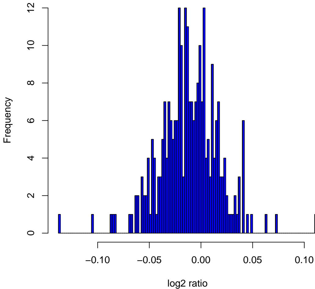
Histogram of \log_2 ratios in 270 HapMap samples at clone Chr6tp-19F5
