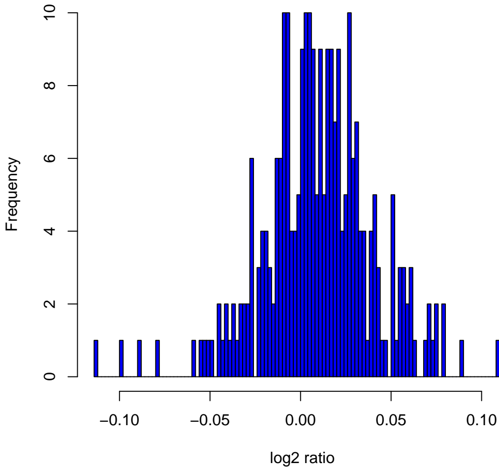
Histogram of log 2 ratios in 270 HapMap samples at clone Chr6tp-19G3
