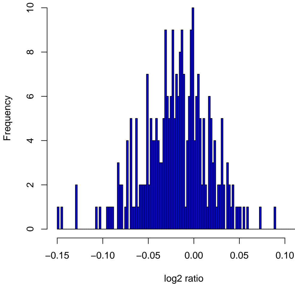
Histogram of \log_2 ratios in 270 HapMap samples at clone Chr6tp-19G7
