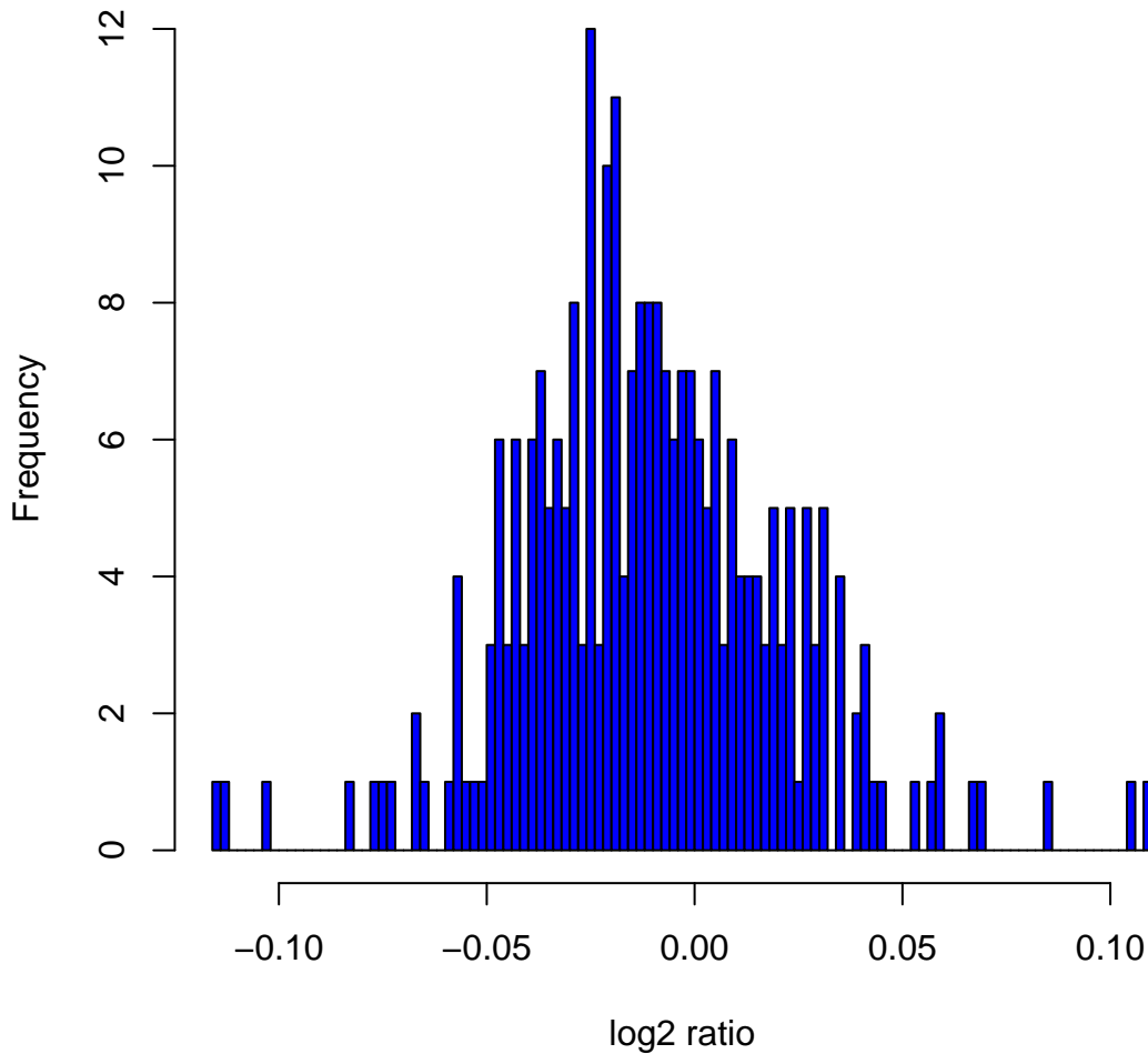
Histogram of \log_2 ratios in 270 HapMap samples at clone Chr6tp-1A8
