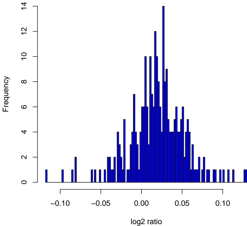
Histogram of log 2 ratios in 270 HapMap samples at clone Chr6tp-1A9
