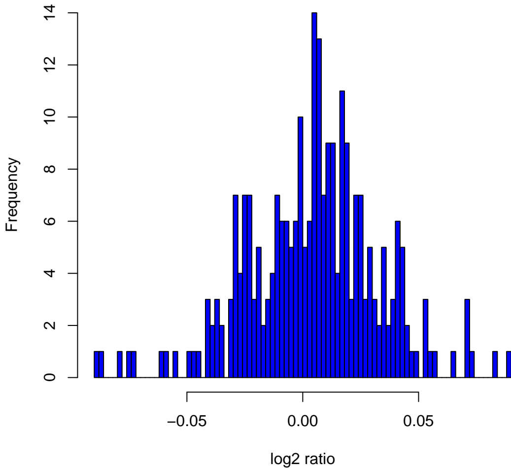
Histogram of log 2 ratios in 270 HapMap samples at clone Chr6tp-1B1
