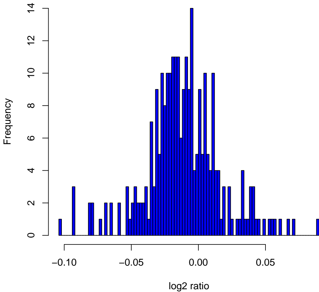
Histogram of log 2 ratios in 270 HapMap samples at clone Chr6tp-1B10
