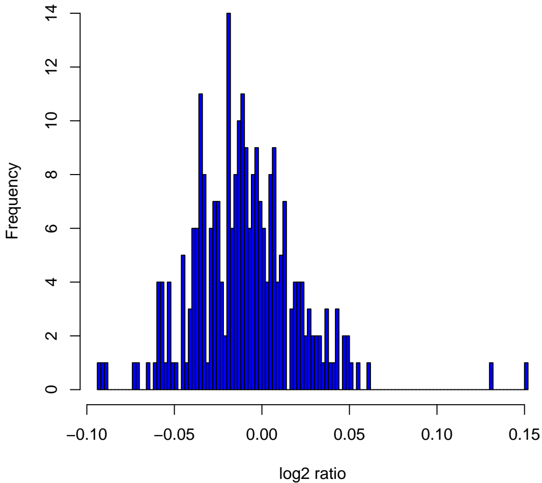
Histogram of log 2 ratios in 270 HapMap samples at clone Chr6tp-1B12
