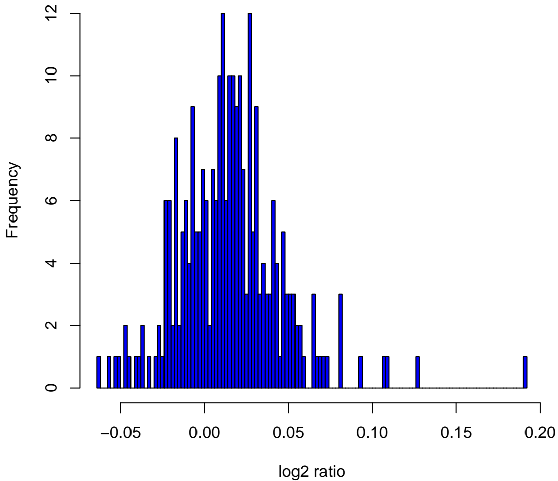
Histogram of log 2 ratios in 270 HapMap samples at clone Chr6tp-1D5
