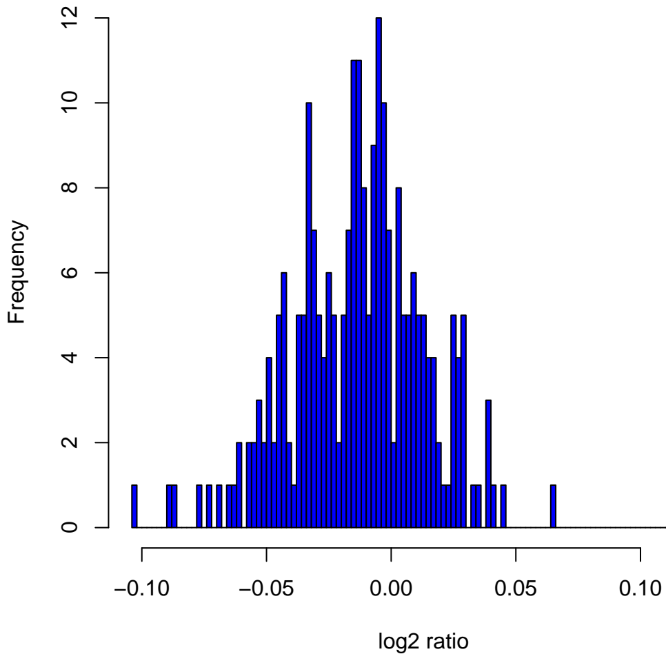
Histogram of log 2 ratios in 270 HapMap samples at clone Chr6tp-1D6
