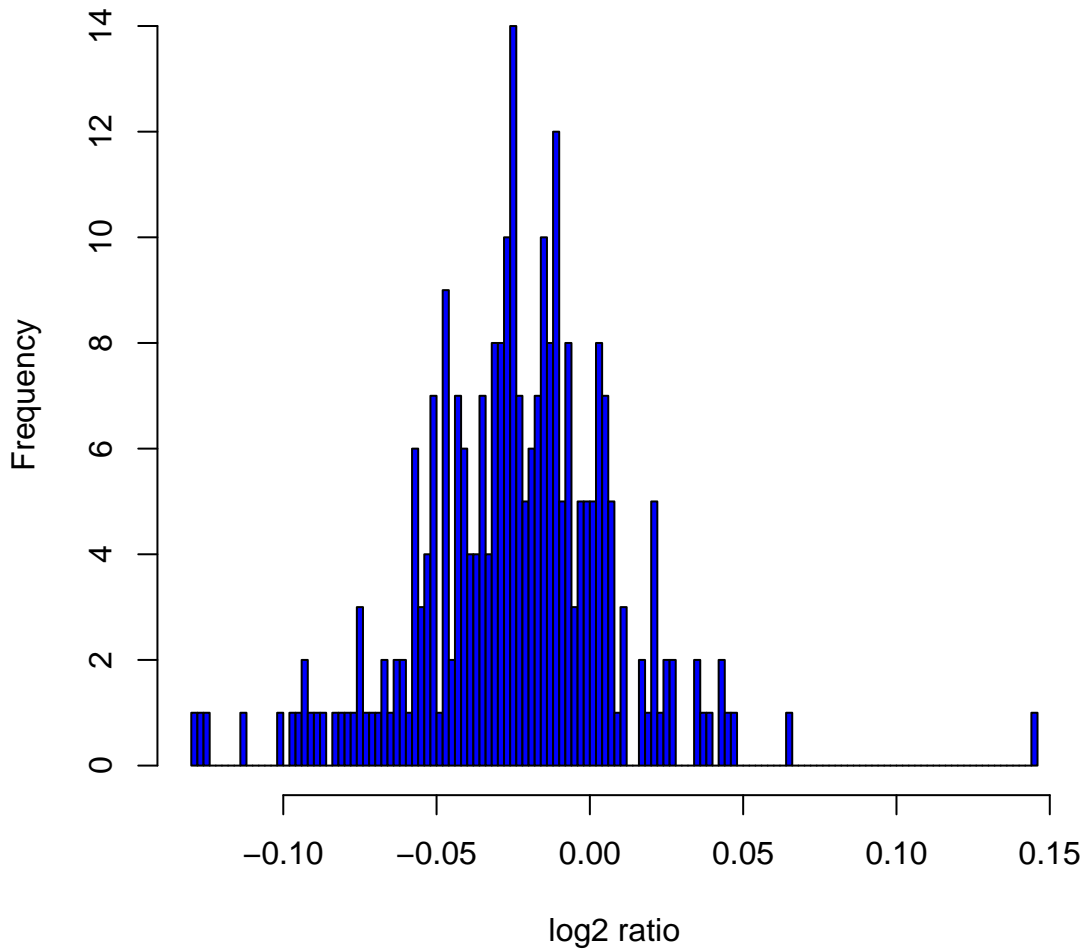
Histogram of log 2 ratios in 270 HapMap samples at clone Chr6tp-1D8
