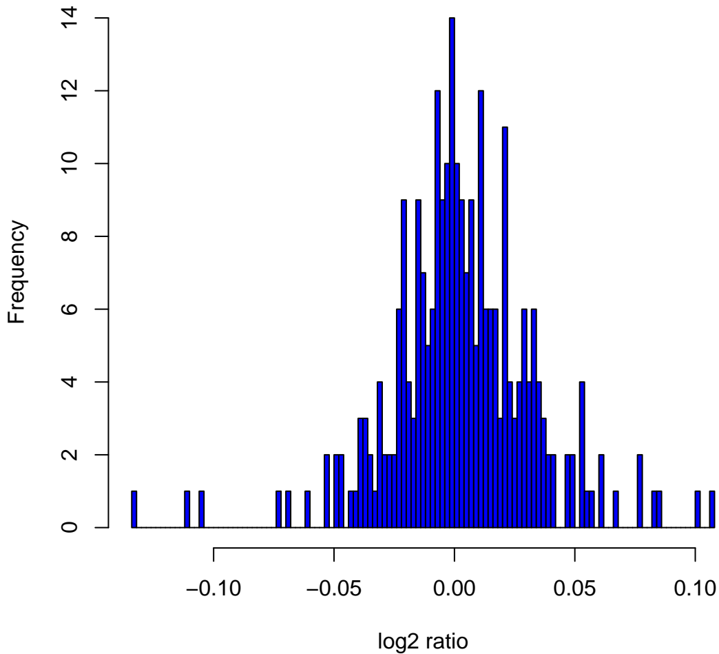
Histogram of log 2 ratios in 270 HapMap samples at clone Chr6tp-1E4
