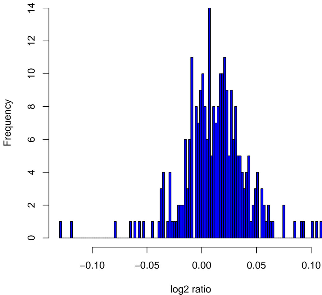
Histogram of log 2 ratios in 270 HapMap samples at clone Chr6tp-1G1
