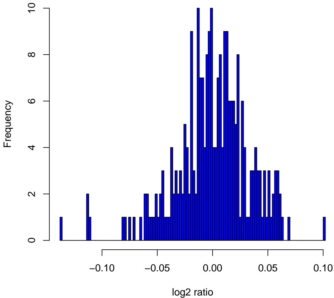
Histogram of log 2 ratios in 270 HapMap samples at clone Chr6tp-20C1
