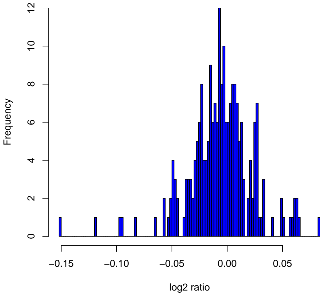
Histogram of log2ratios in 270 HapMap samples at clone Chr6tp-22B10
