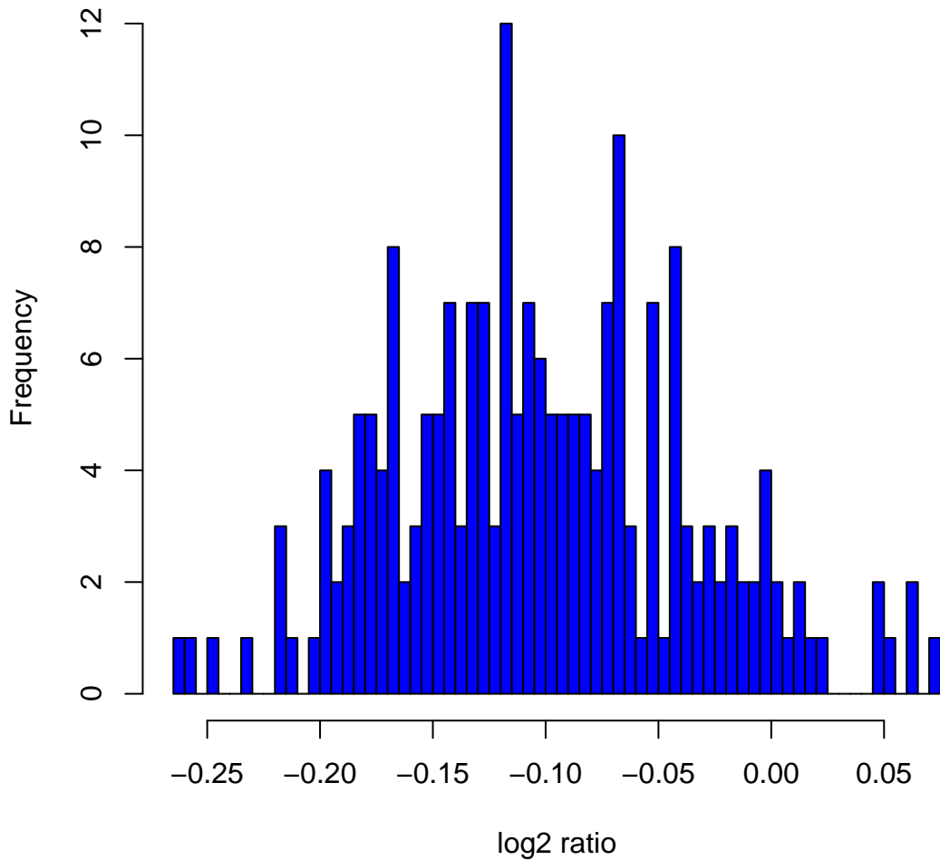
Histogram of log2ratios in 270 HapMap samples at clone Chr6tp-22C12
