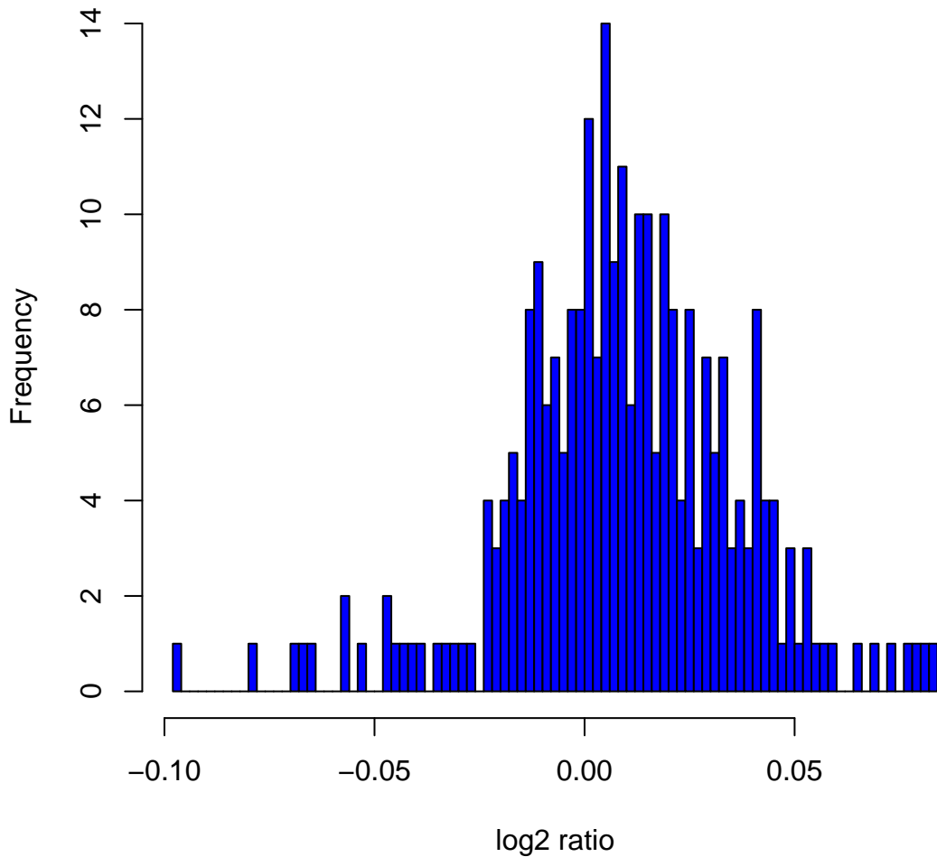
Histogram of \log_2 ratios in 270 HapMap samples at clone Chr6tp-2A4
