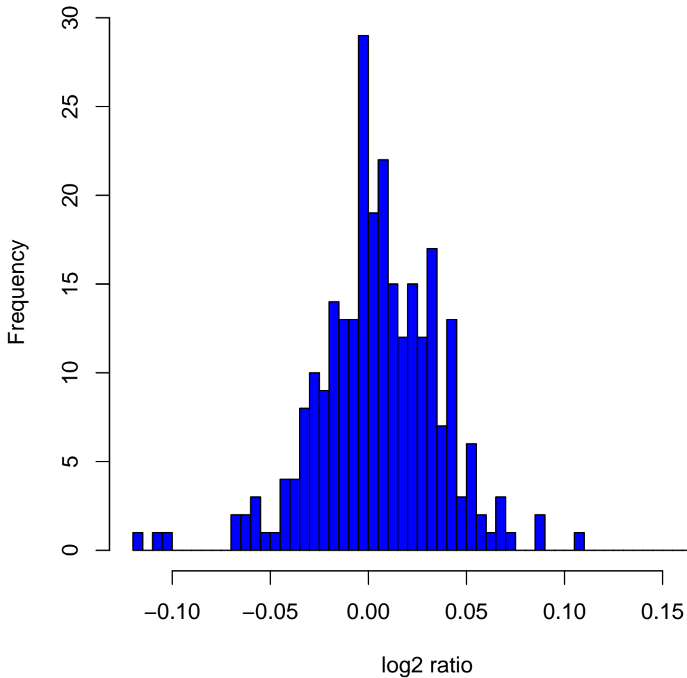
Histogram of log 2 ratios in 270 HapMap samples at clone Chr6tp-2C5
