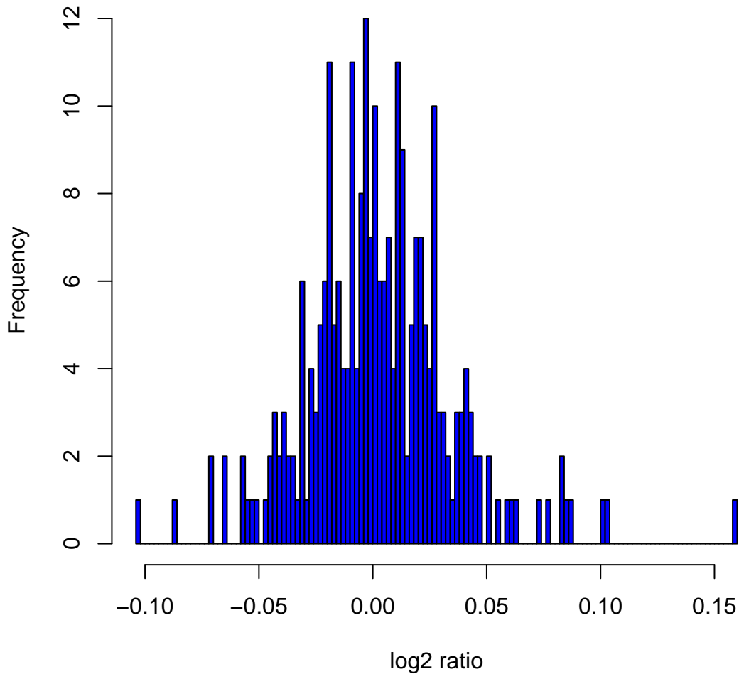
Histogram of log 2 ratios in 270 HapMap samples at clone Chr6tp-2D11
