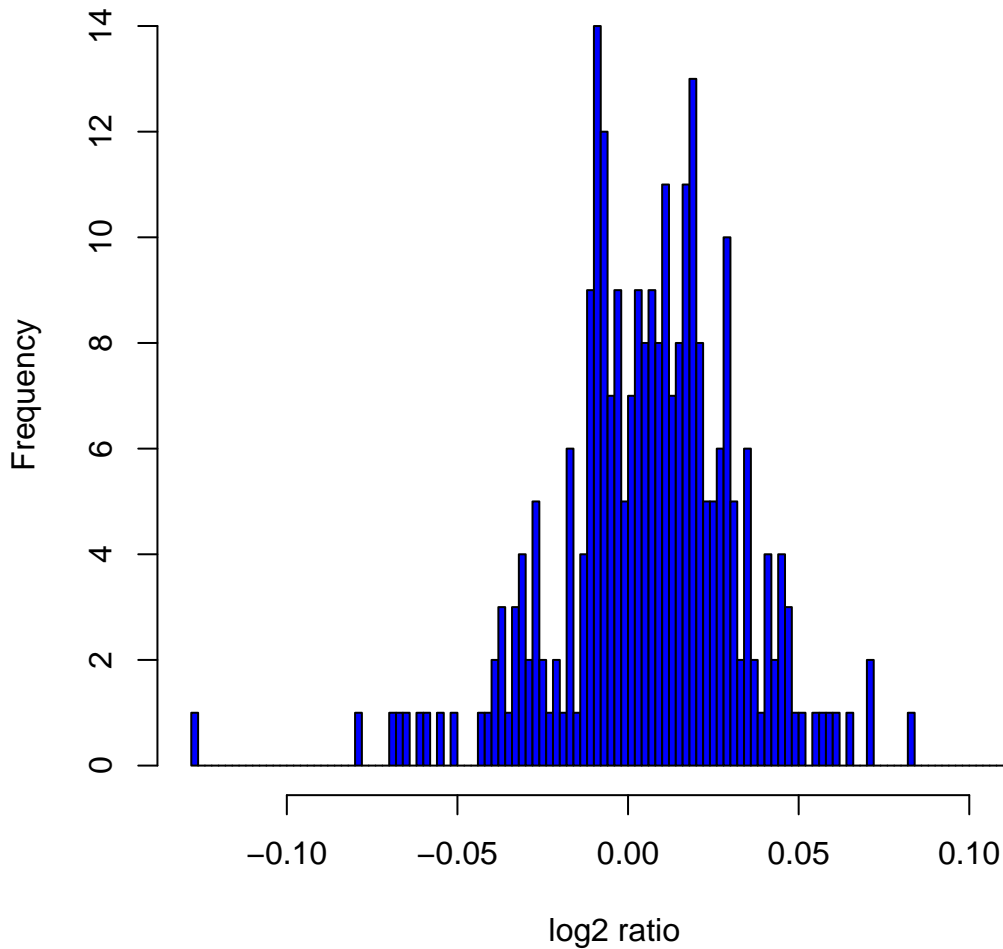
Histogram of log 2 ratios in 270 HapMap samples at clone Chr6tp-2D4
