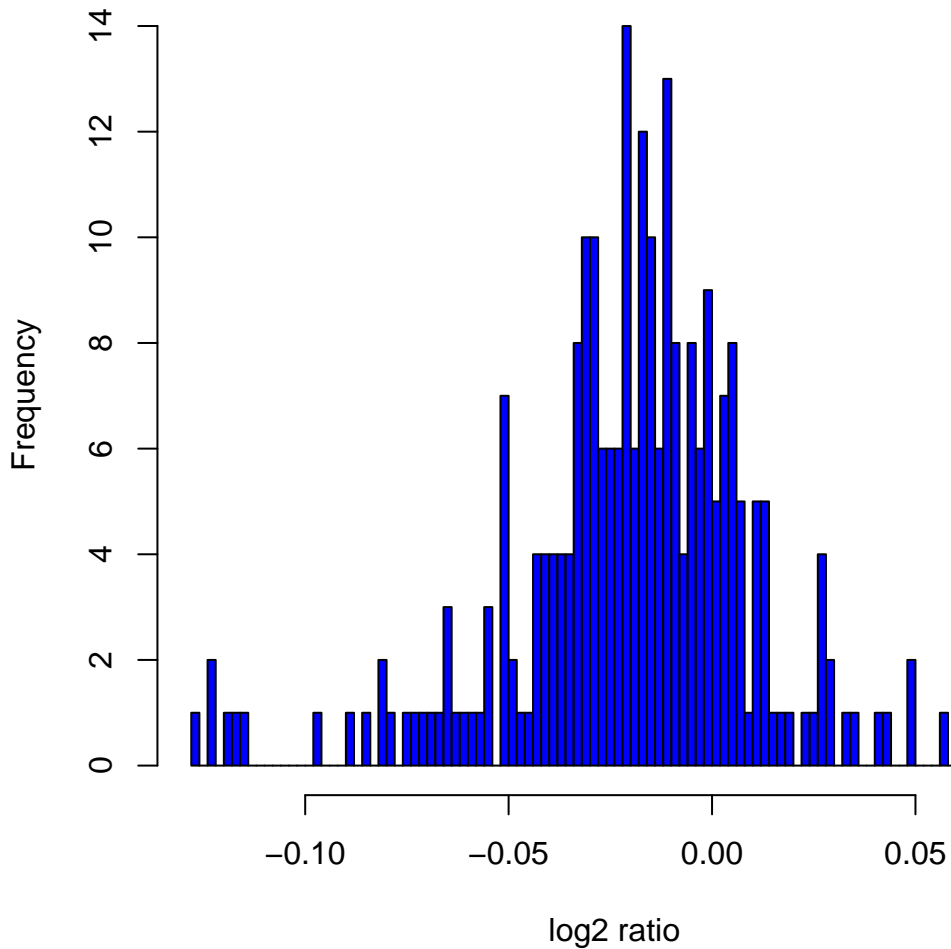
Histogram of \log_2 ratios in 270 HapMap samples at clone Chr6tp-2D7
