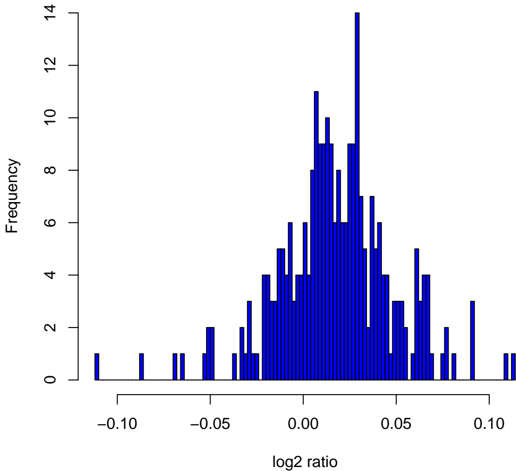
Histogram of log 2 ratios in 270 HapMap samples at clone Chr6tp-2D9
