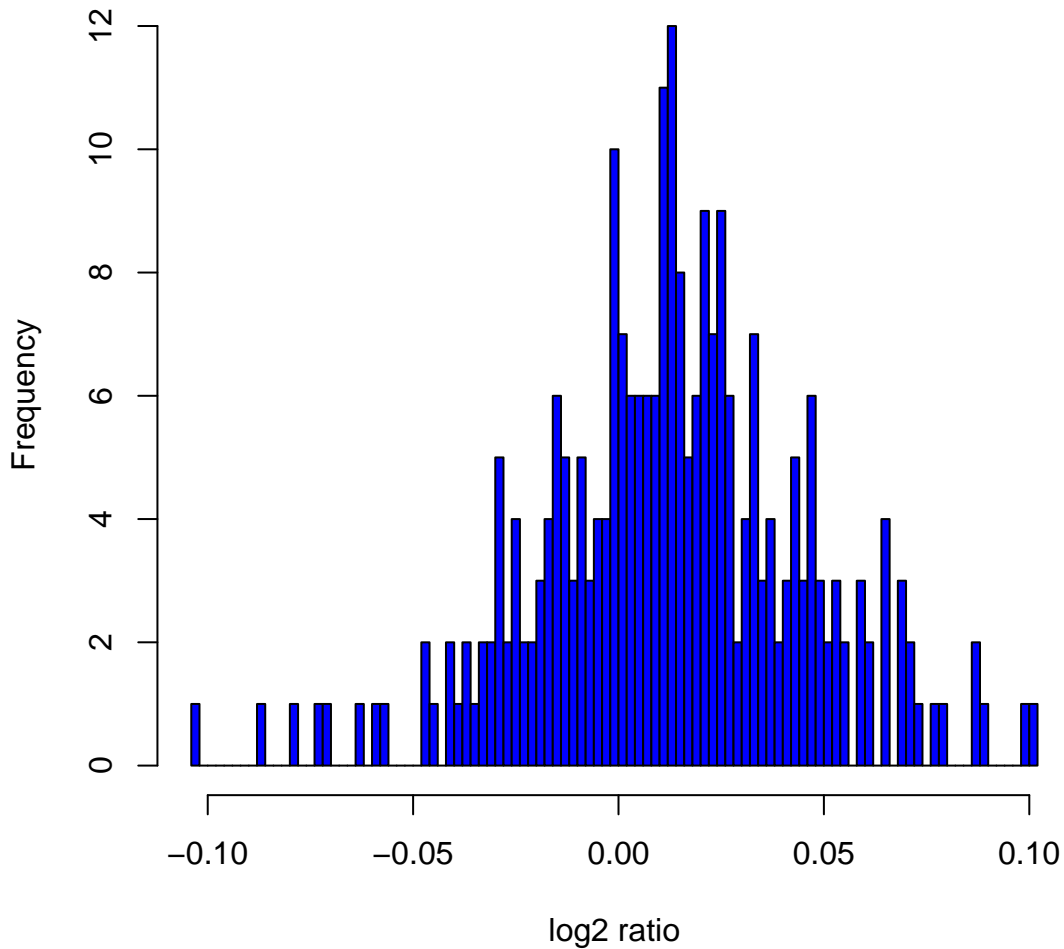
Histogram of \log_2 ratios in 270 HapMap samples at clone Chr6tp-2H1
