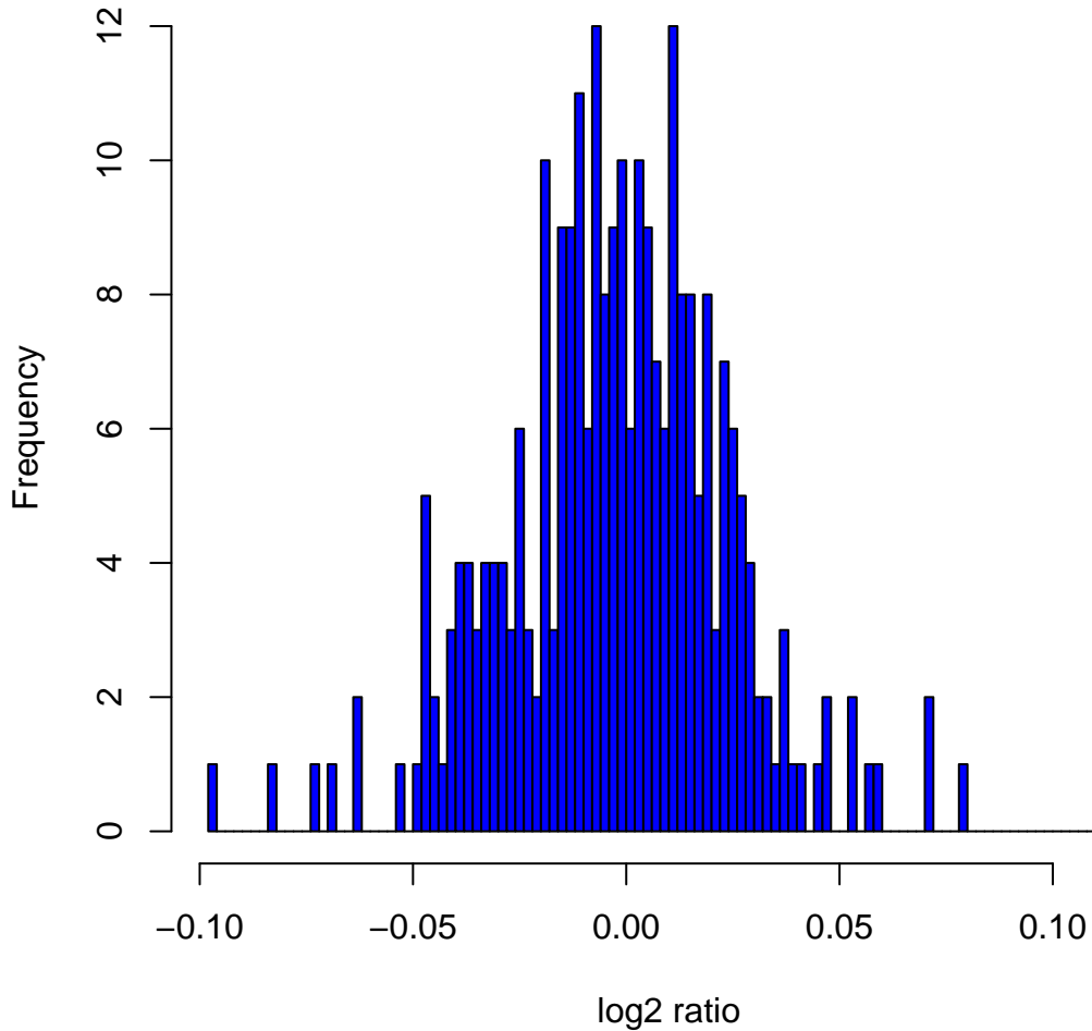
Histogram of log 2 ratios in 270 HapMap samples at clone Chr6tp-2H12
