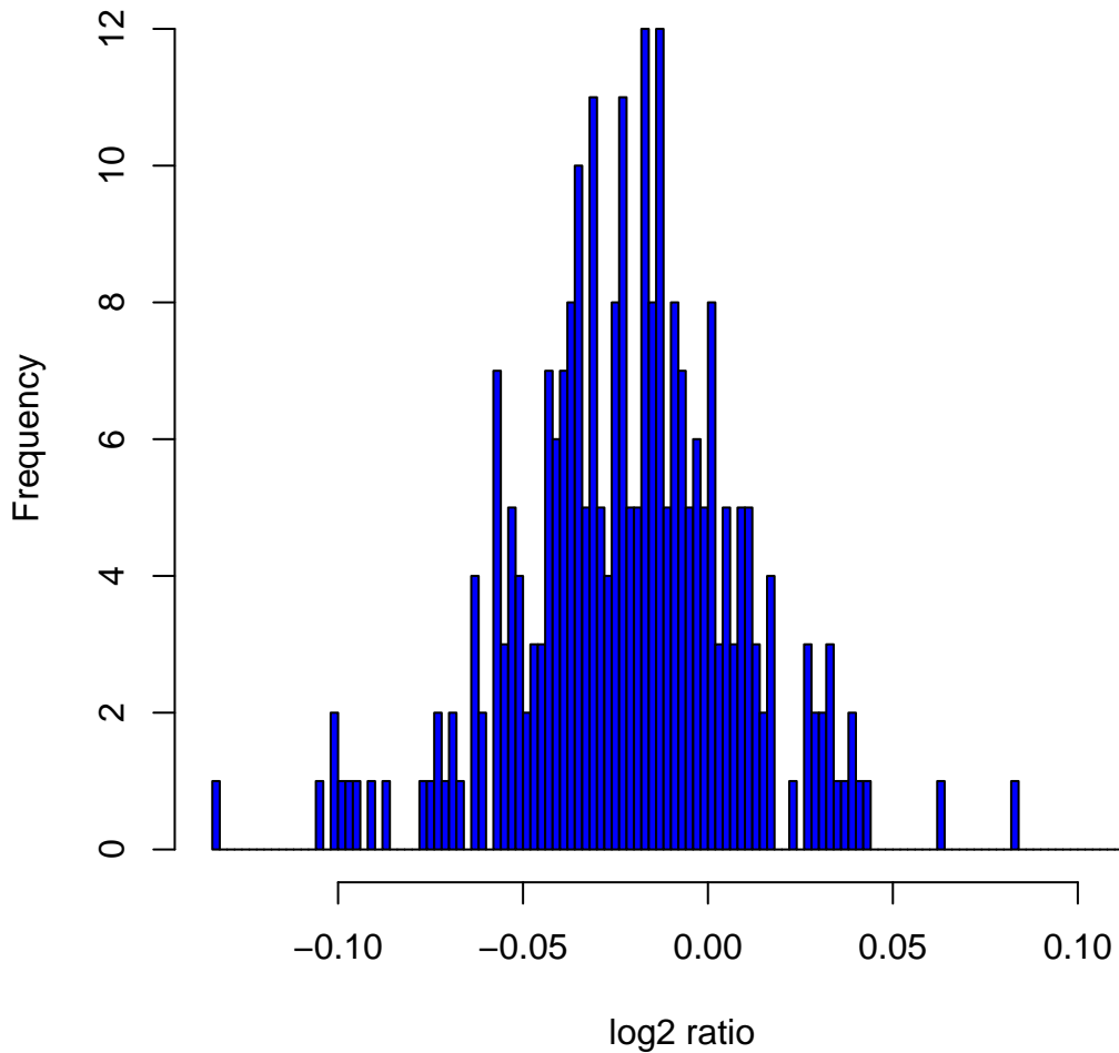
Histogram of log2ratios in 270 HapMap samples at clone Chr6tp-2H3
