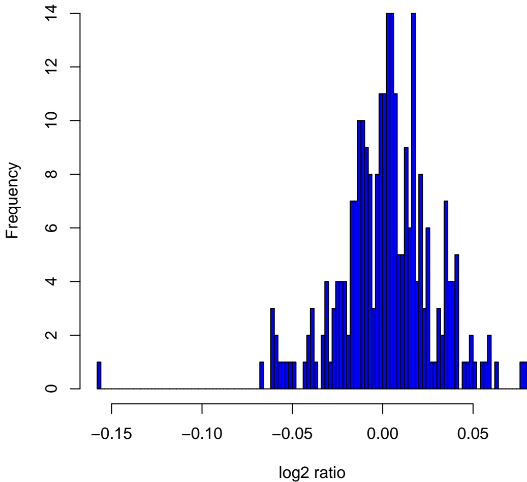
Histogram of log 2 ratios in 270 HapMap samples at clone Chr6tp-2H4
