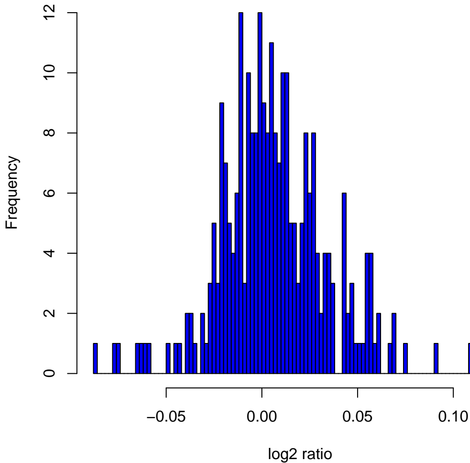
Histogram of \log_2 ratios in 270 HapMap samples at clone Chr6tp-3C2
