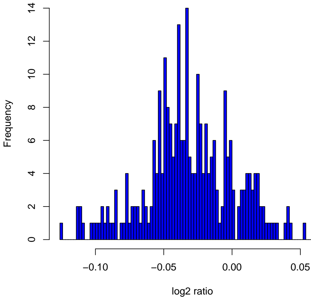
Histogram of log 2 ratios in 270 HapMap samples at clone Chr6tp-3C8
