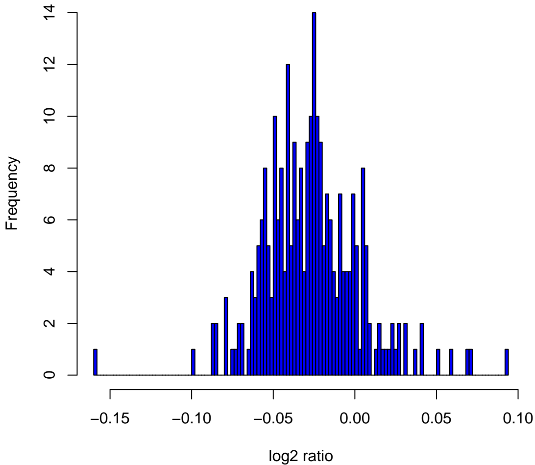
Histogram of log 2 ratios in 270 HapMap samples at clone Chr6tp-3C9
