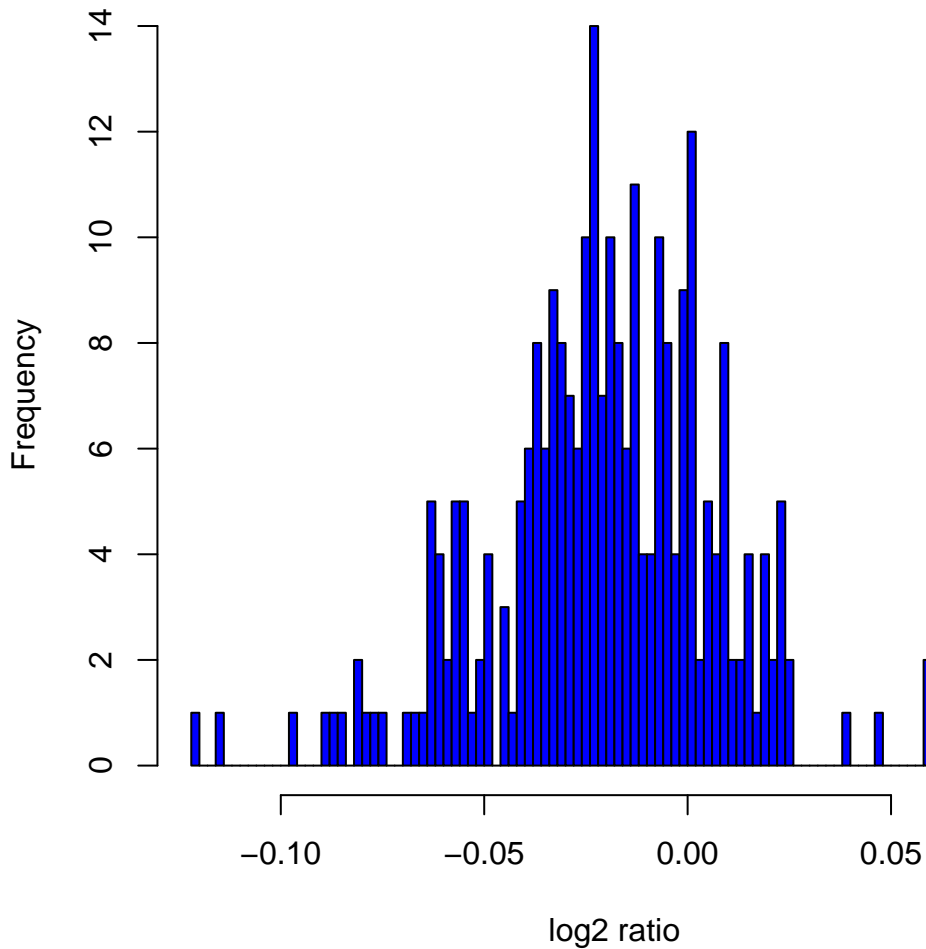
Histogram of \log_2 ratios in 270 HapMap samples at clone Chr6tp-3D3
