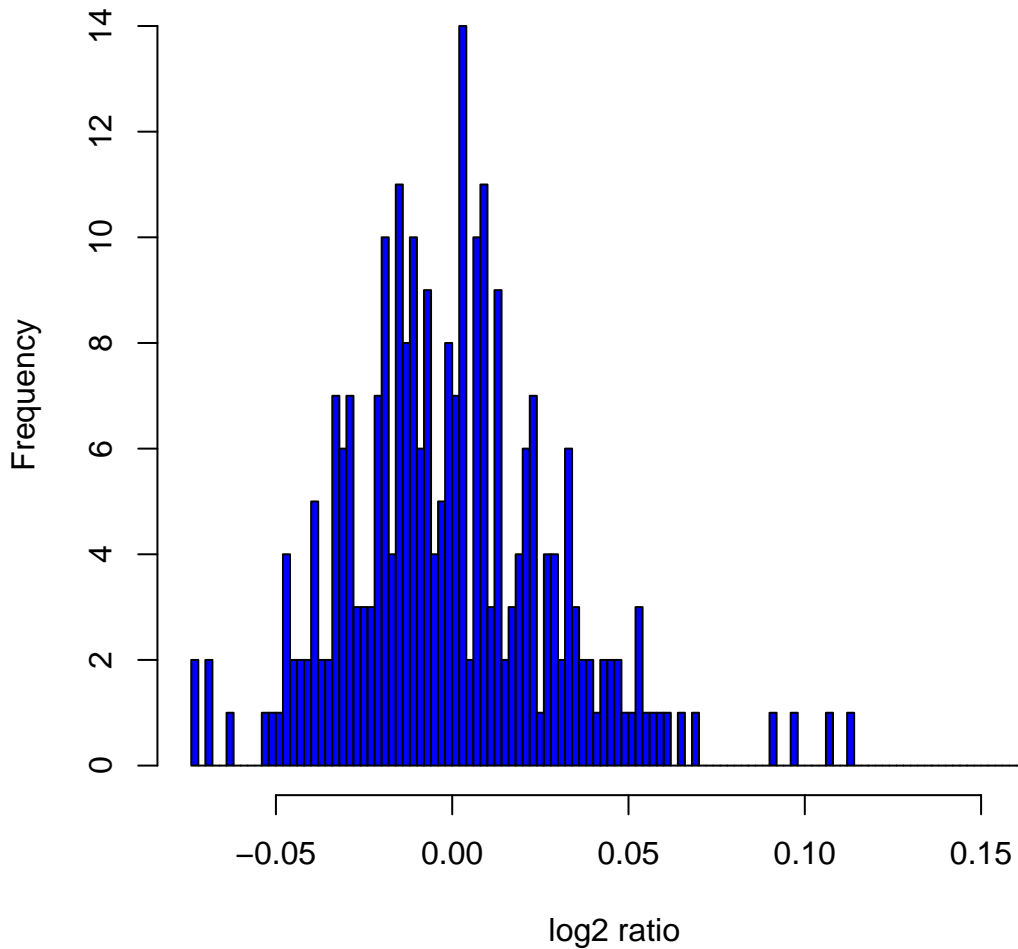
Histogram of \log_2 ratios in 270 HapMap samples at clone Chr6tp-3D5
