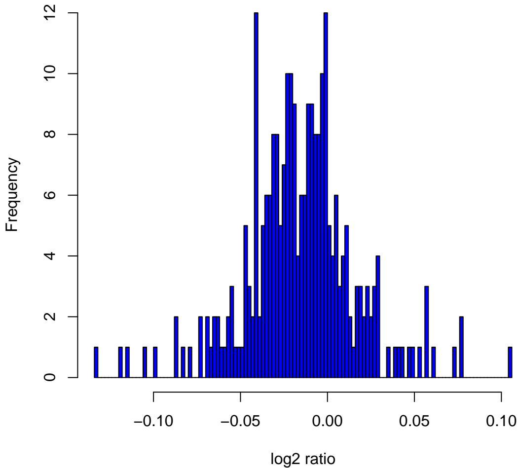
Histogram of \log_2 ratios in 270 HapMap samples at clone Chr6tp-3D9
