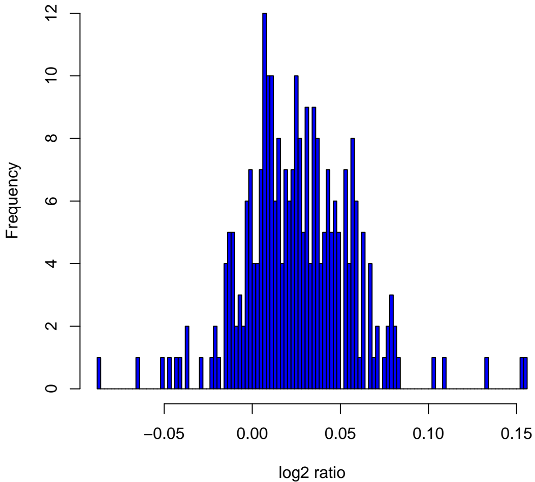
Histogram of log2ratios in 270 HapMap samples at clone Chr6tp-3E4
