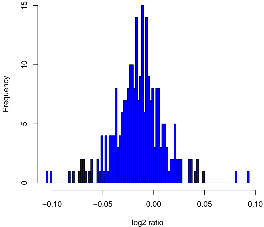
Histogram of log2ratios in 270 HapMap samples at clone Chr6tp-3F1
