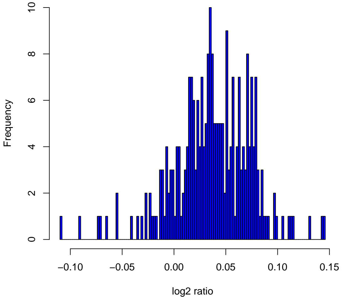
Histogram of log2ratios in 270 HapMap samples at clone Chr6tp-3F8
