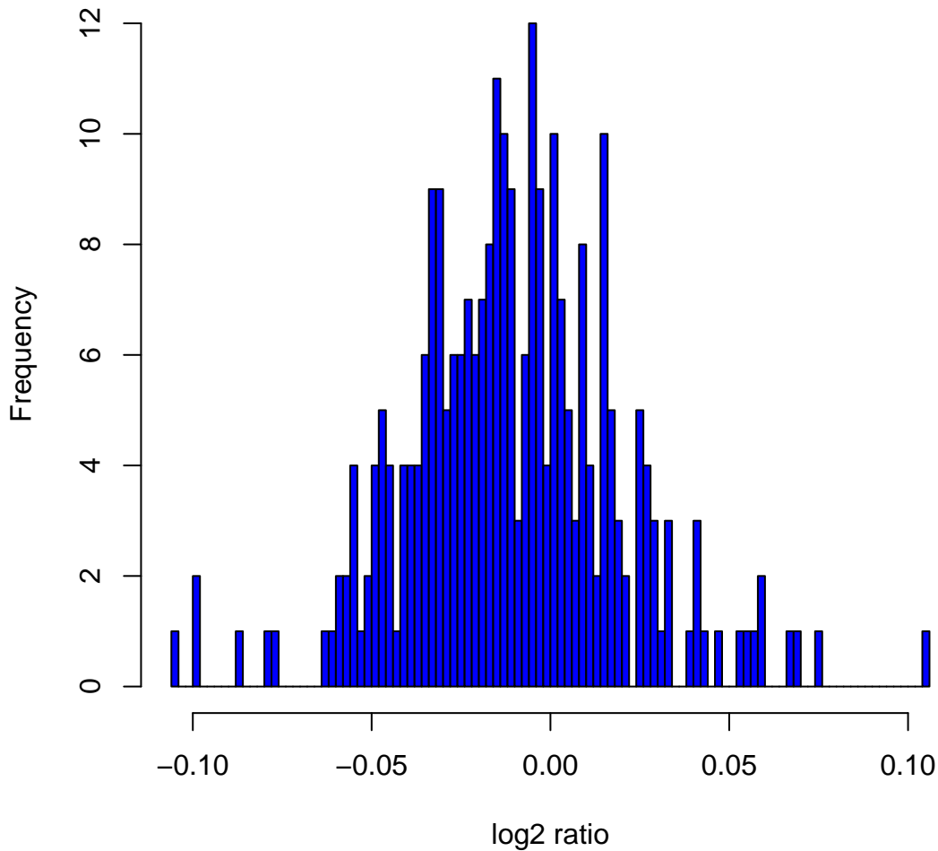
Histogram of log 2 ratios in 270 HapMap samples at clone Chr6tp-3G10
