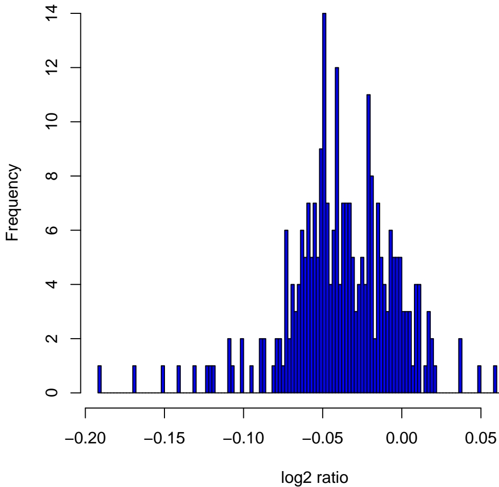
Histogram of log2ratios in 270 HapMap samples at clone Chr6tp-3G12
